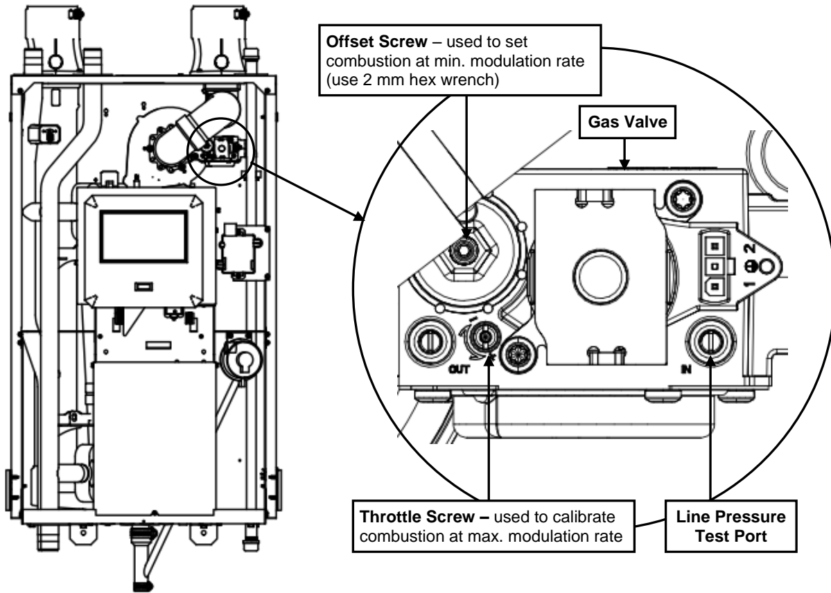
Figure 2 Gas Valve Venturi Assembly
